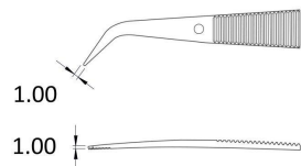
Dimensions mm
