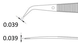
Dimensions inch
